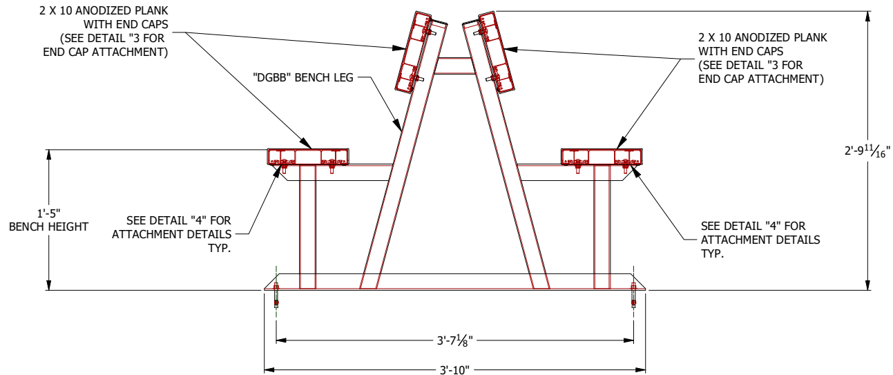
CONCRETE ANCHOR OPTION SEE DETAIL "2"
